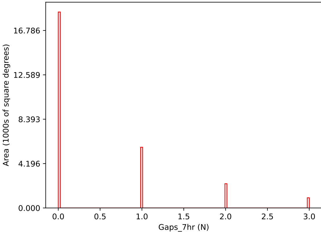
too_elab_r32_d2_ugrizy_v3.4_10yrs i band: Gaps_7hr
