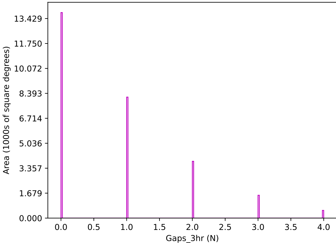
too_elab_r32_d2_ugrizy_v3.4_10yrs z band: Gaps_3hr
