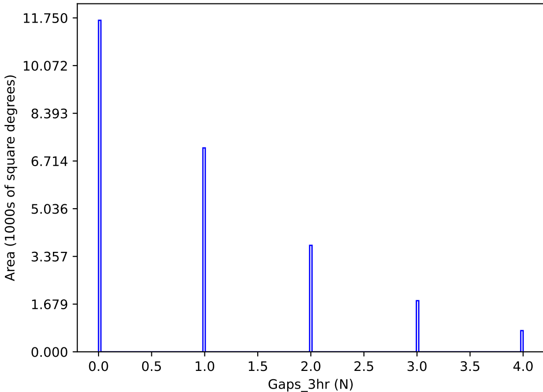
too_elab_r32_d2_ugrizy_v3.4_10yrs y band: Gaps_3hr
