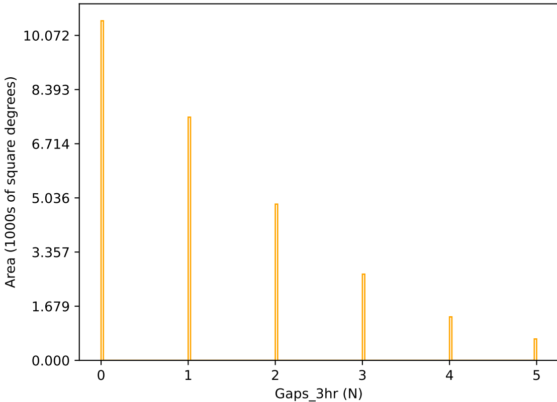
too_elab_r32_d2_ugrizy_v3.4_10yrs r band: Gaps_3hr
