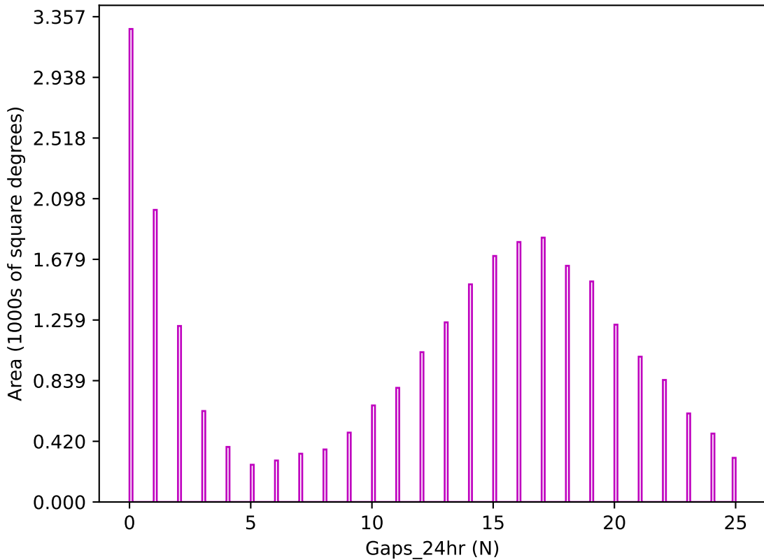
too_elab_r32_d2_ugrizy_v3.4_10yrs z band: Gaps_24hr
