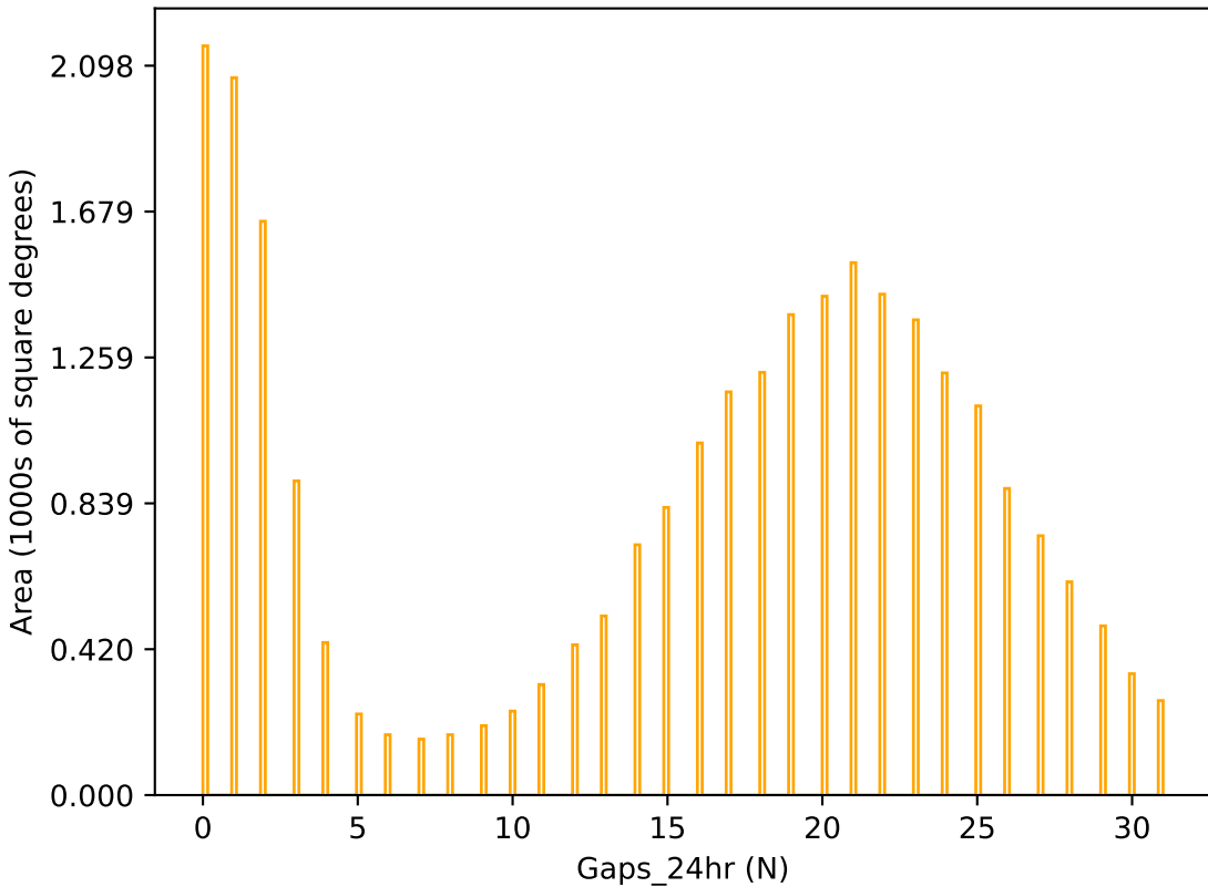
too_elab_r32_d2_ugrizy_v3.4_10yrs r band: Gaps_24hr
