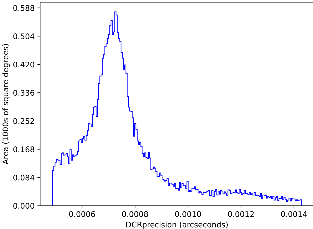
too_elab_r32_d2_ugrizy_v3.4_10yrs : DCRprecision
