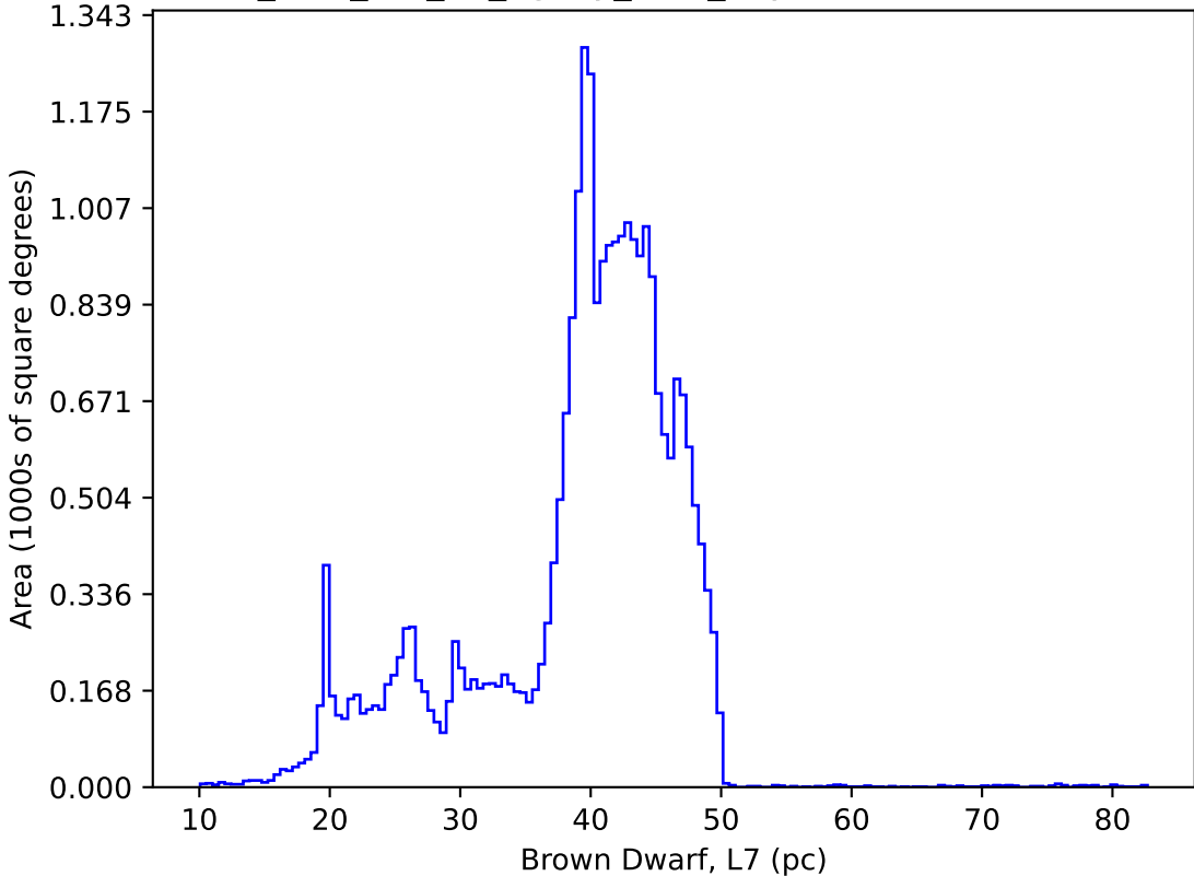
too_elab_r32_d2_ugrizy_v3.4_10yrs : Brown Dwarf, L7
