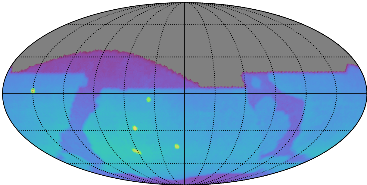
too_elab_r32_d2_ugrizy_v3.4_10yrs : Brown Dwarf, L4
