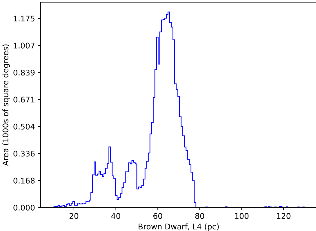
too_elab_r32_d2_ugrizy_v3.4_10yrs : Brown Dwarf, L4
