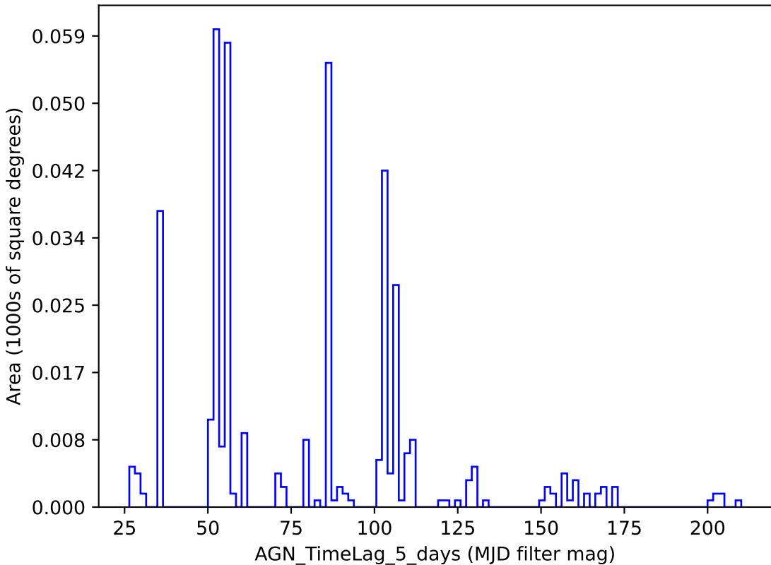
too_elab_r32_d2_ugrizy_v3.4_10yrs y band: AGN_TimeLag_5_days
