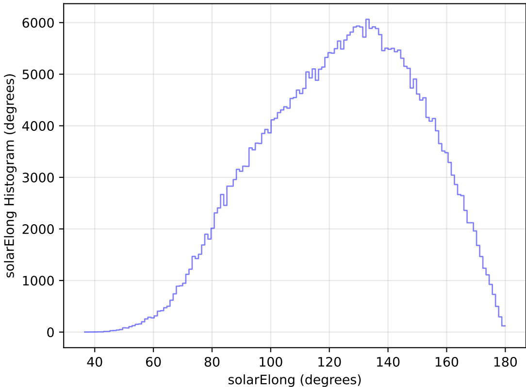
too_elab_r32_d2_ugrizy_v3.4_10yrs WFD y band: solarElong Histogram
