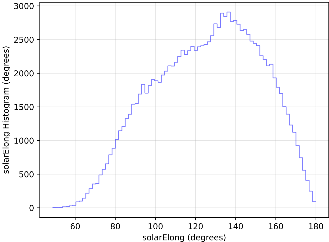
too_elab_r32_d2_ugrizy_v3.4_10yrs WFD u band: solarElong Histogram
