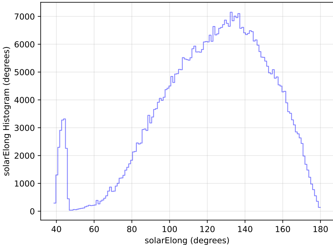
too_elab_r32_d2_ugrizy_v3.4_10yrs WFD r band: solarElong Histogram
