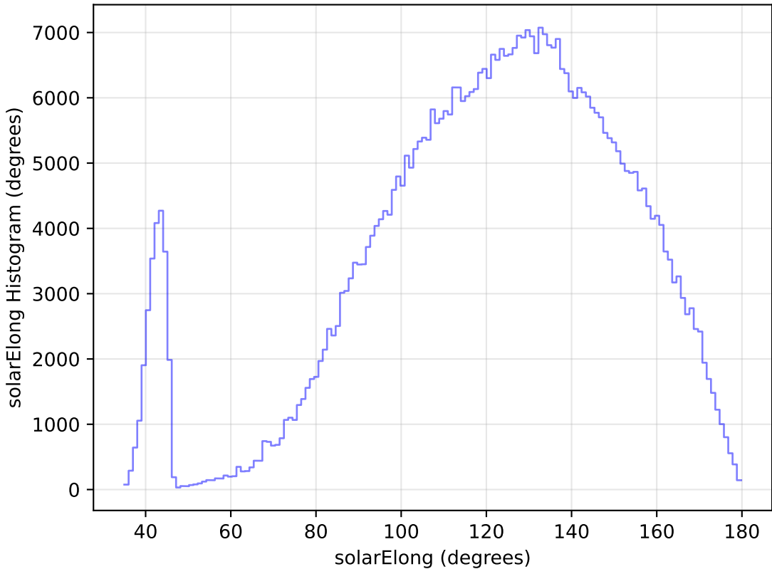
too_elab_r32_d2_ugrizy_v3.4_10yrs WFD i band: solarElong Histogram
