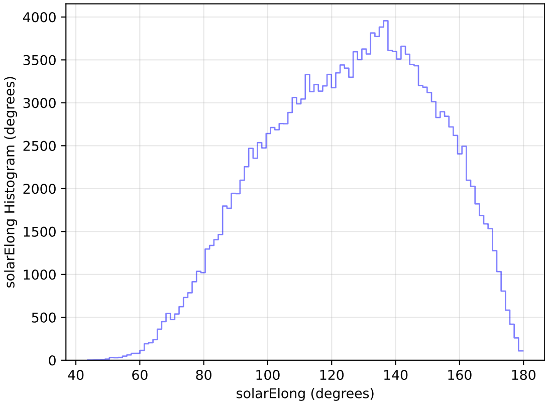
too_elab_r32_d2_ugrizy_v3.4_10yrs WFD g band: solarElong Histogram
