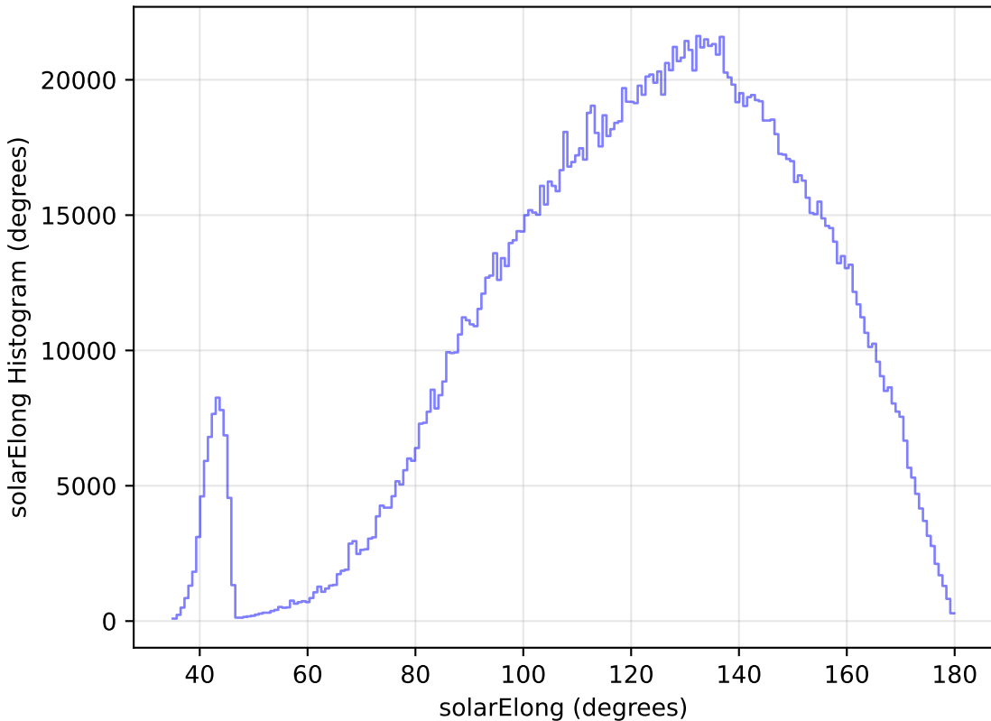
too_elab_r32_d2_ugrizy_v3.4_10yrs WFD all bands: solarElong Histogram
