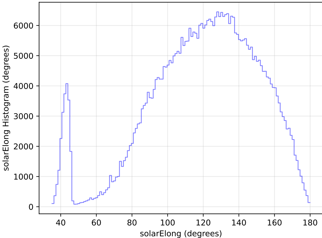
too_elab_r32_d2_ugrizy_v3.4_10yrs All sky z band: solarElong Histogram
