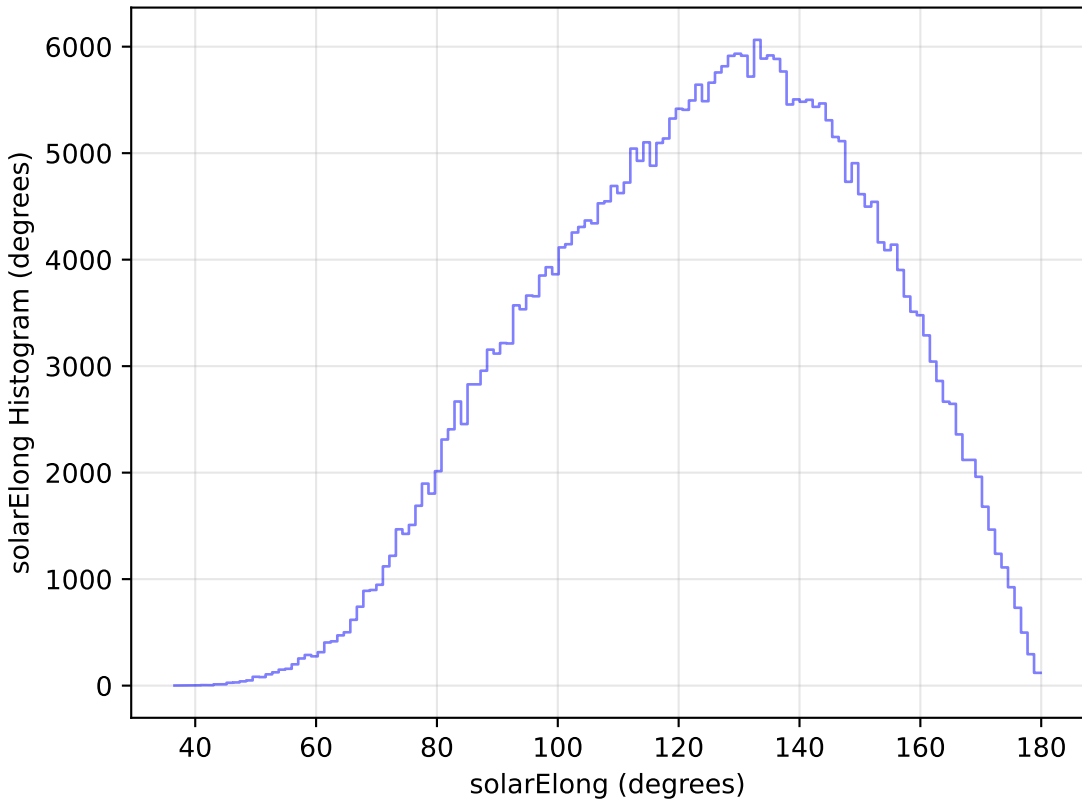
too_elab_r32_d2_ugrizy_v3.4_10yrs All sky y band: solarElong Histogram
