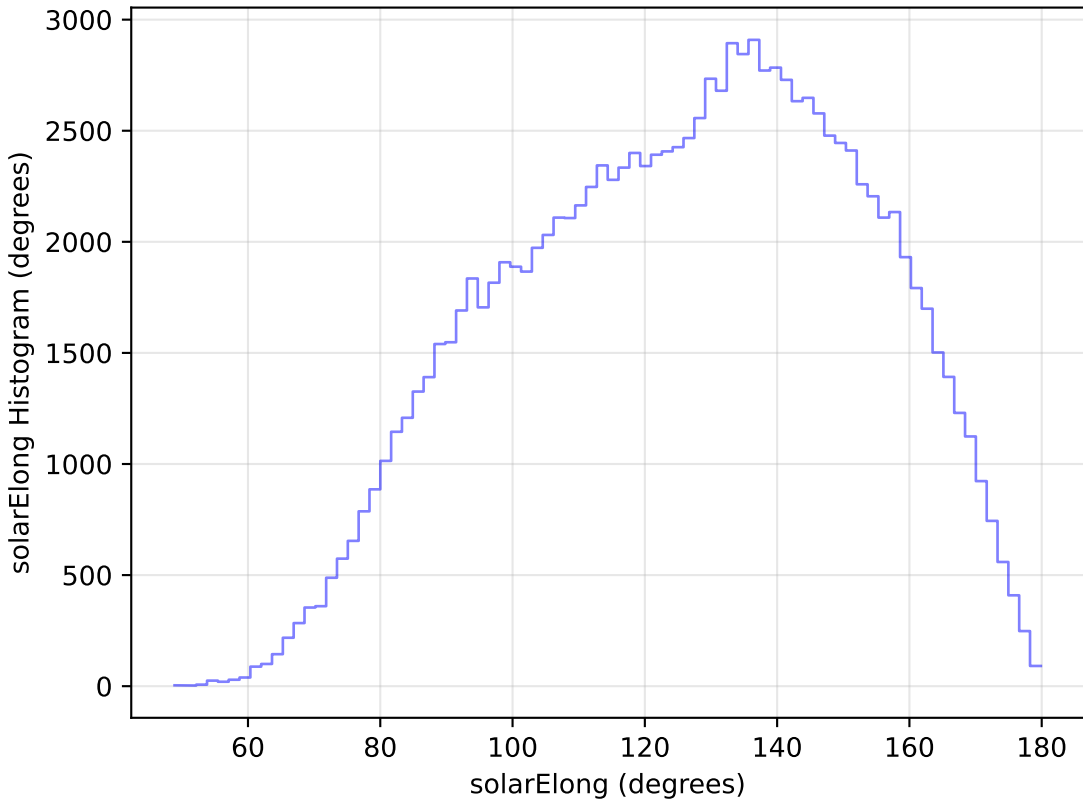
too_elab_r32_d2_ugrizy_v3.4_10yrs All sky u band: solarElong Histogram
