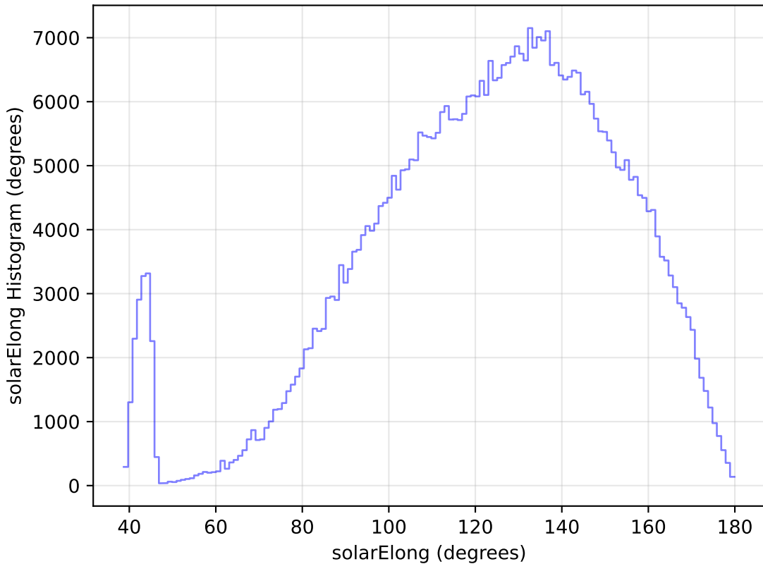
too_elab_r32_d2_ugrizy_v3.4_10yrs All sky r band: solarElong Histogram
