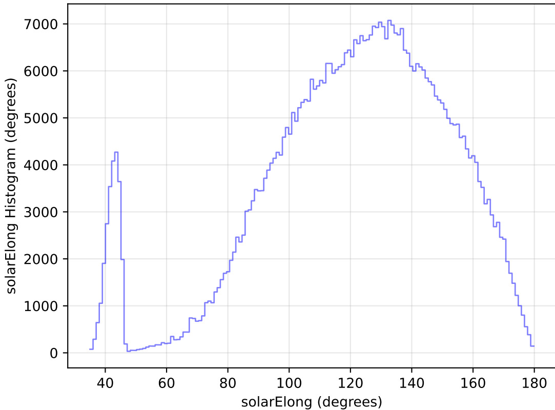
too_elab_r32_d2_ugrizy_v3.4_10yrs All sky i band: solarElong Histogram
