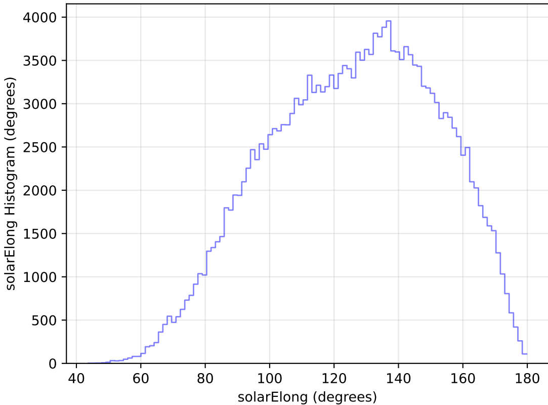
too_elab_r32_d2_ugrizy_v3.4_10yrs All sky g band: solarElong Histogram
