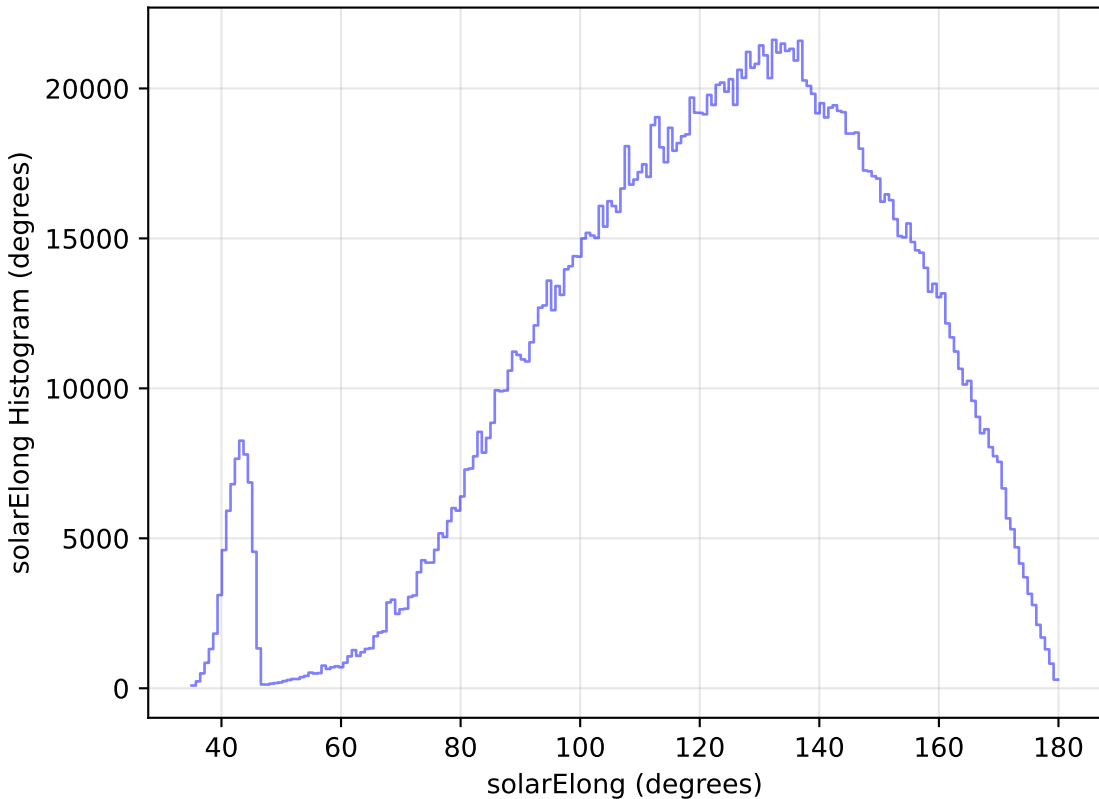
too_elab_r32_d2_ugrizy_v3.4_10yrs All sky all bands: solarElong Histogram
