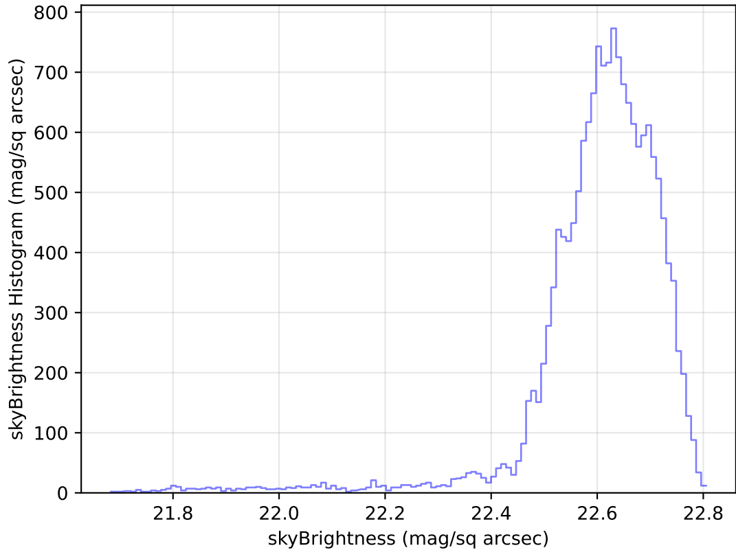
too_elab_r32_d2_ugrizy_v3.4_10yrs Yr 1 u band: skyBrightness Histogram
