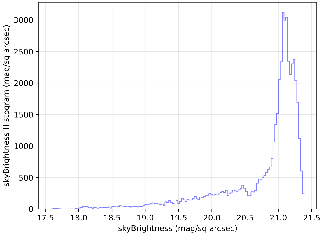
too_elab_r32_d2_ugrizy_v3.4_10yrs Yr 1 r band: skyBrightness Histogram
