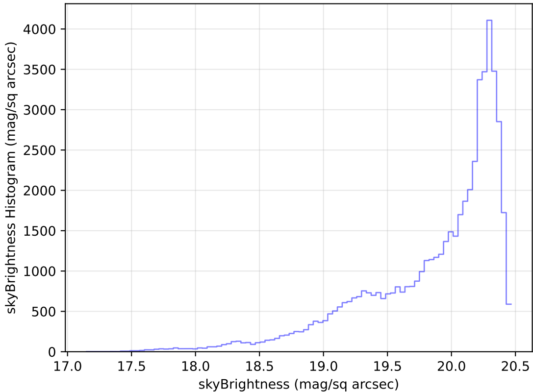
too_elab_r32_d2_ugrizy_v3.4_10yrs Yr 1 i band: skyBrightness Histogram
