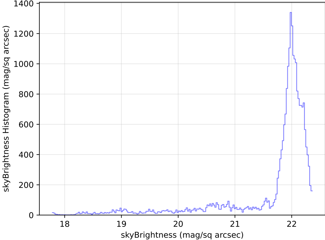
too_elab_r32_d2_ugrizy_v3.4_10yrs Yr 1 g band: skyBrightness Histogram
