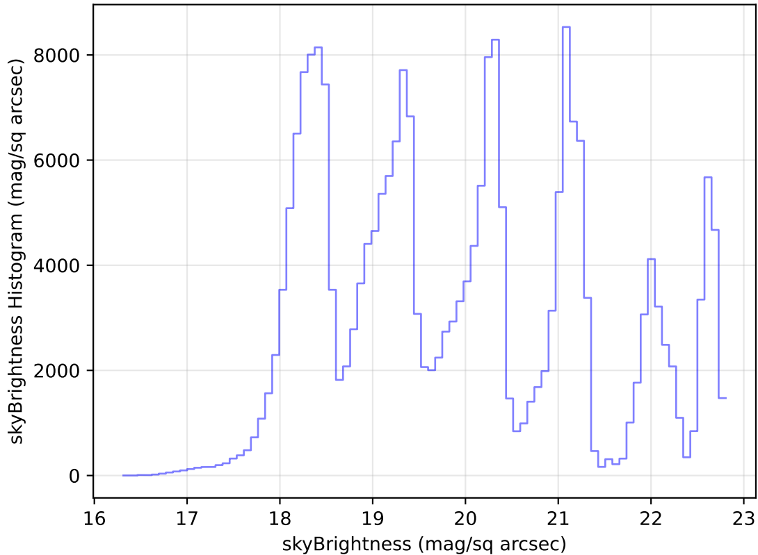
too_elab_r32_d2_ugrizy_v3.4_10yrs Yr 1 all bands: skyBrightness Histogram
