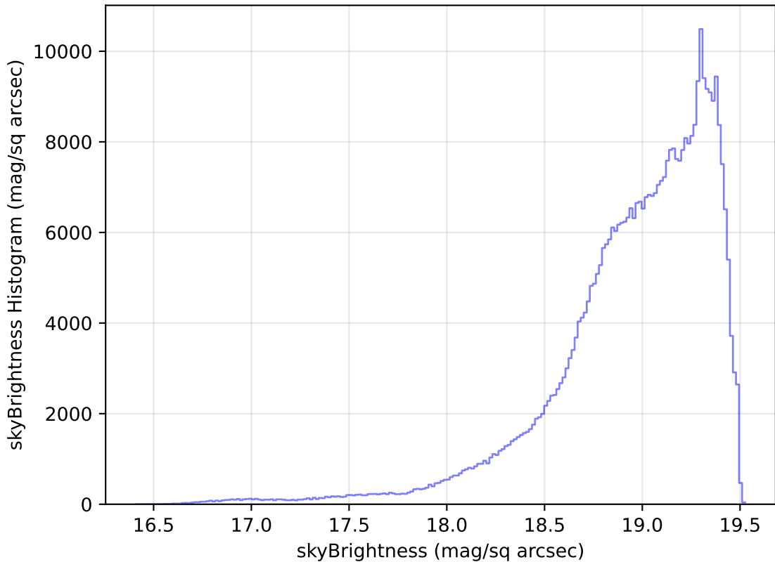
too_elab_r32_d2_ugrizy_v3.4_10yrs WFD z band: skyBrightness Histogram
