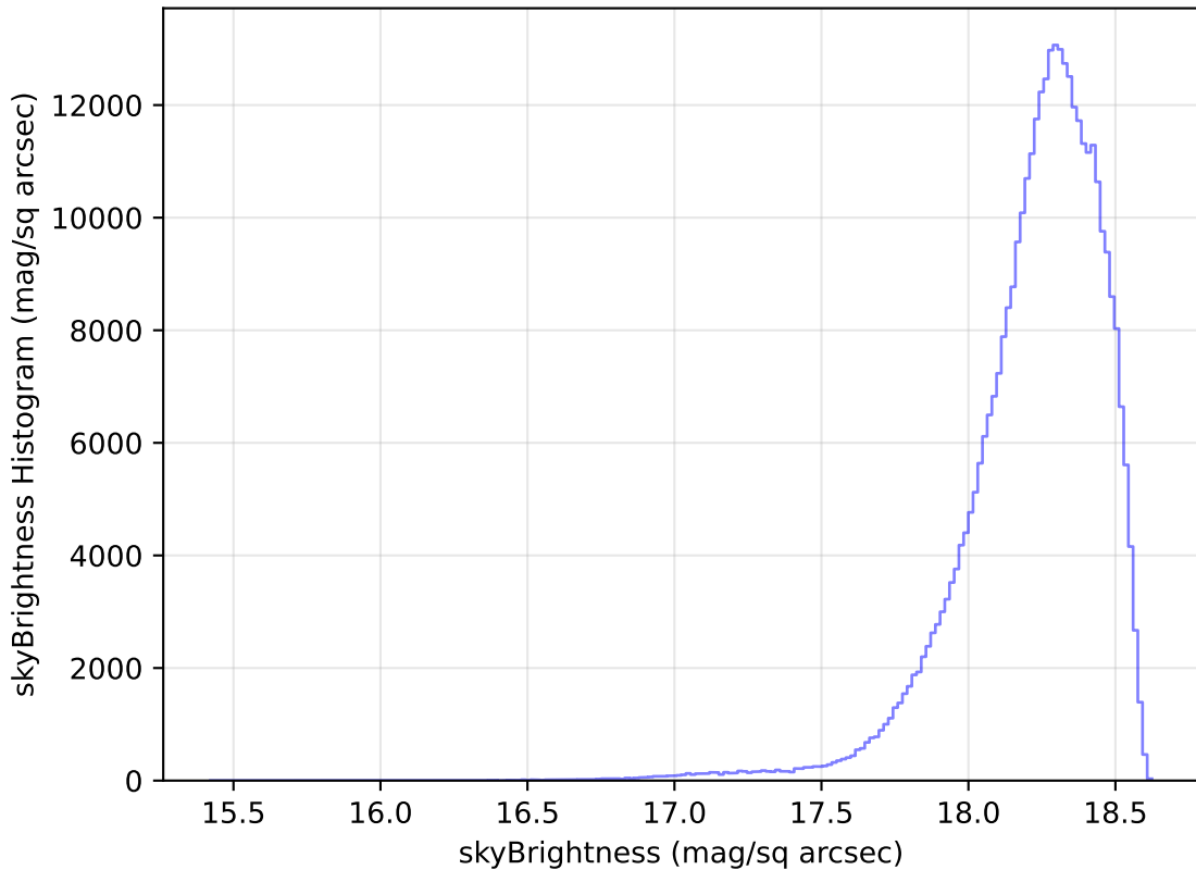
too_elab_r32_d2_ugrizy_v3.4_10yrs WFD y band: skyBrightness Histogram
