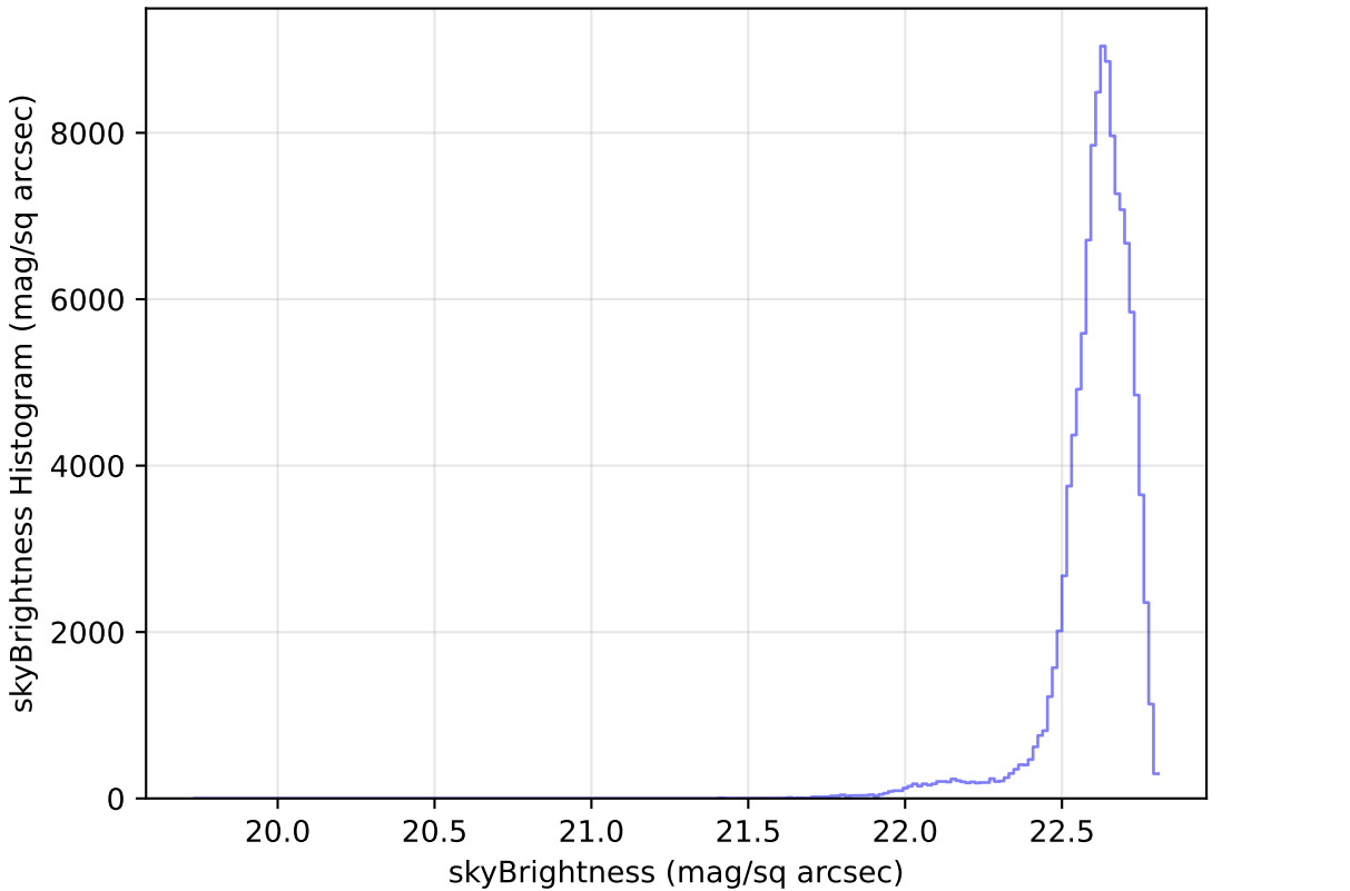
too_elab_r32_d2_ugrizy_v3.4_10yrs WFD u band: skyBrightness Histogram
