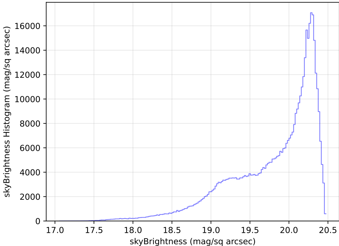
too_elab_r32_d2_ugrizy_v3.4_10yrs WFD i band: skyBrightness Histogram
