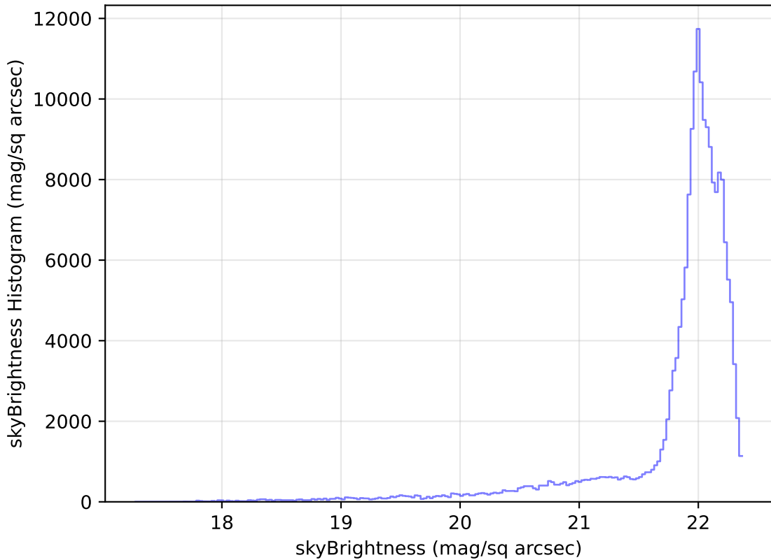
too_elab_r32_d2_ugrizy_v3.4_10yrs WFD g band: skyBrightness Histogram
