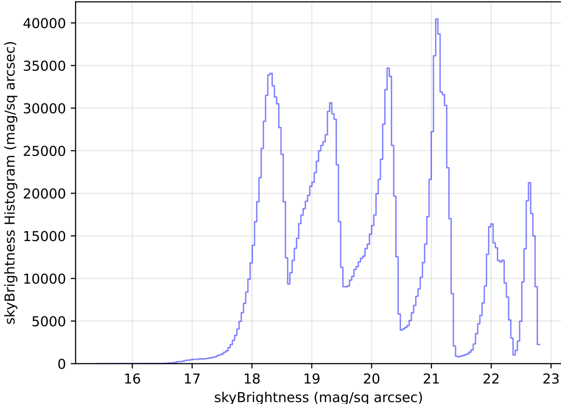
too_elab_r32_d2_ugrizy_v3.4_10yrs WFD all bands: skyBrightness Histogram
