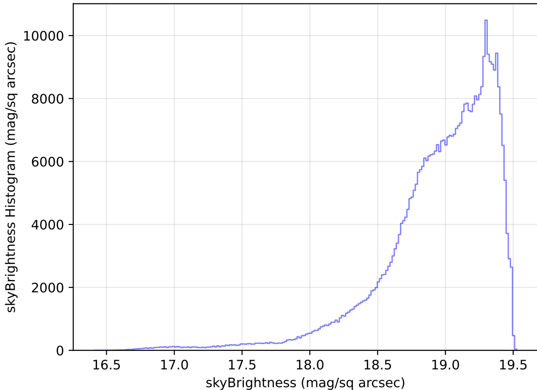
too_elab_r32_d2_ugrizy_v3.4_10yrs All sky z band: skyBrightness Histogram
