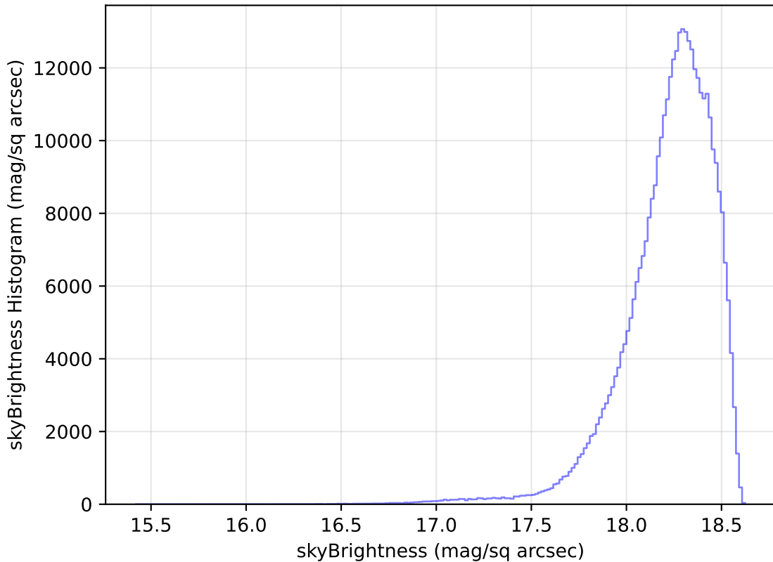
too_elab_r32_d2_ugrizy_v3.4_10yrs All sky y band: skyBrightness Histogram
