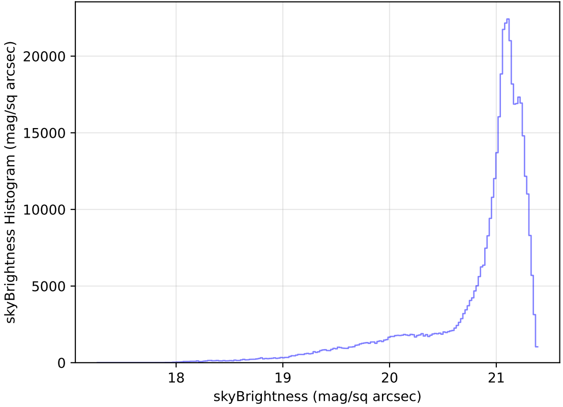
too_elab_r32_d2_ugrizy_v3.4_10yrs All sky r band: skyBrightness Histogram
