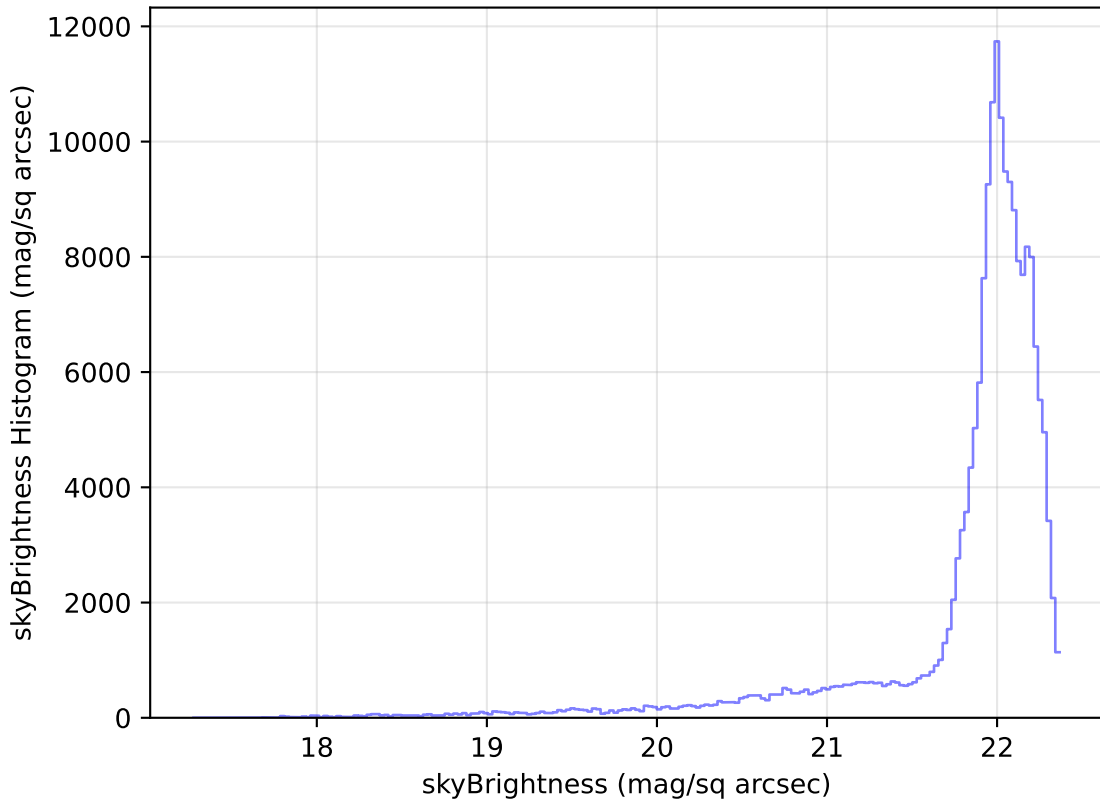
too_elab_r32_d2_ugrizy_v3.4_10yrs All sky g band: skyBrightness Histogram
