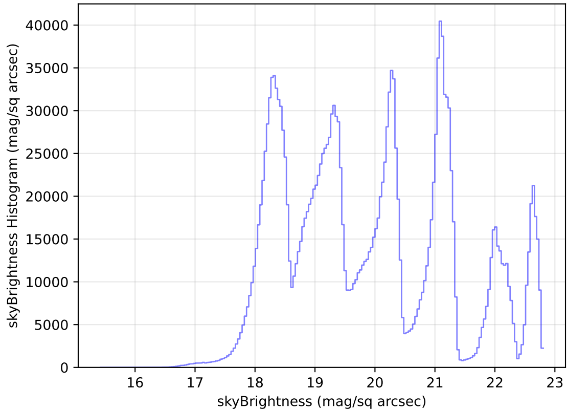
too_elab_r32_d2_ugrizy_v3.4_10yrs All sky all bands: skyBrightness Histogram
