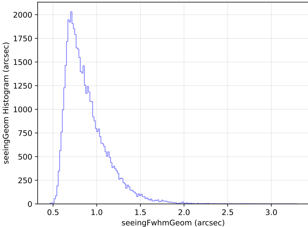
too_elab_r32_d2_ugrizy_v3.4_10yrs Yr 1 r band: seeingGeom Histogram
