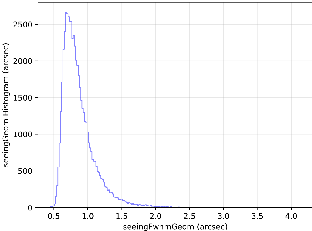
too_elab_r32_d2_ugrizy_v3.4_10yrs Yr 1 i band: seeingGeom Histogram
