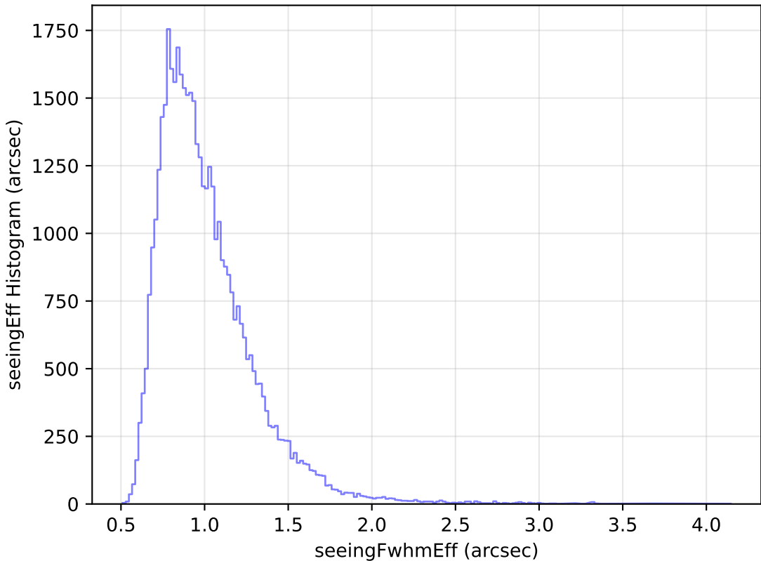
too_elab_r32_d2_ugrizy_v3.4_10yrs Yr 1 z band: seeingEff Histogram
