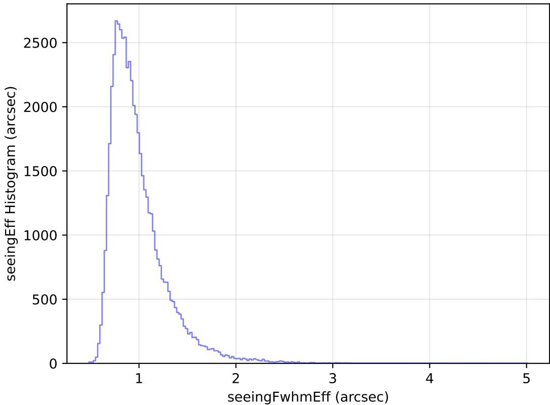
too_elab_r32_d2_ugrizy_v3.4_10yrs Yr 1 i band: seeingEff Histogram
