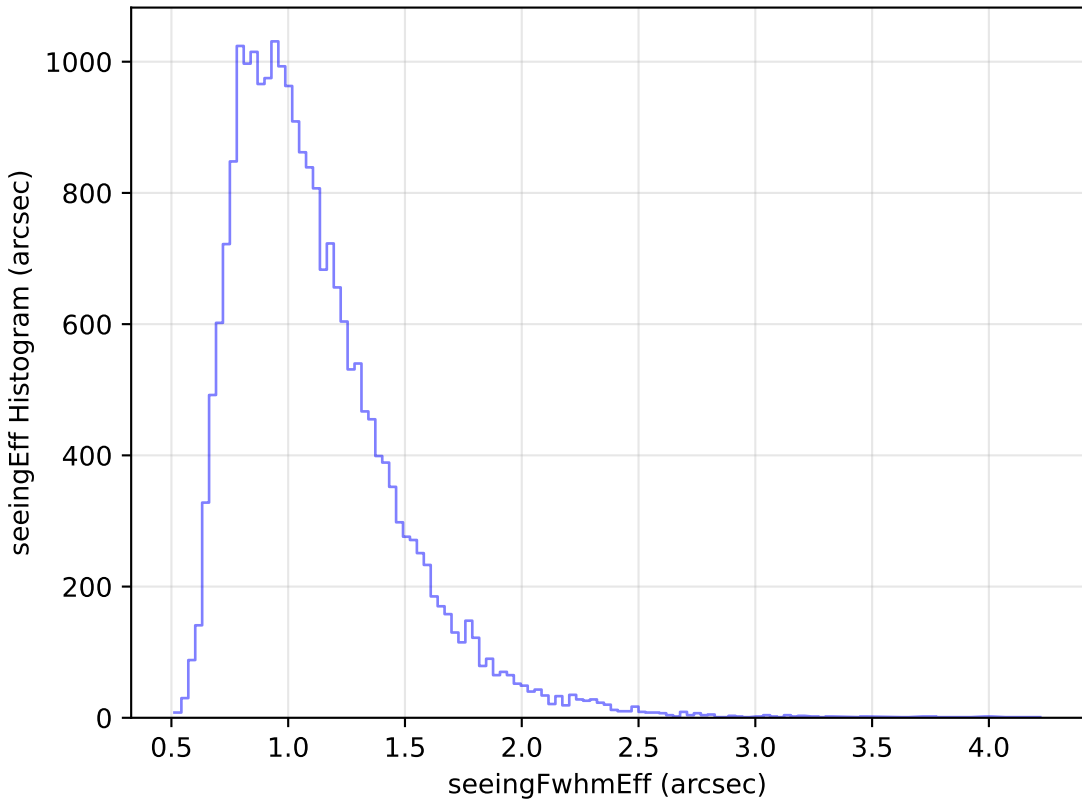
too_elab_r32_d2_ugrizy_v3.4_10yrs Yr 1 g band: seeingEff Histogram
