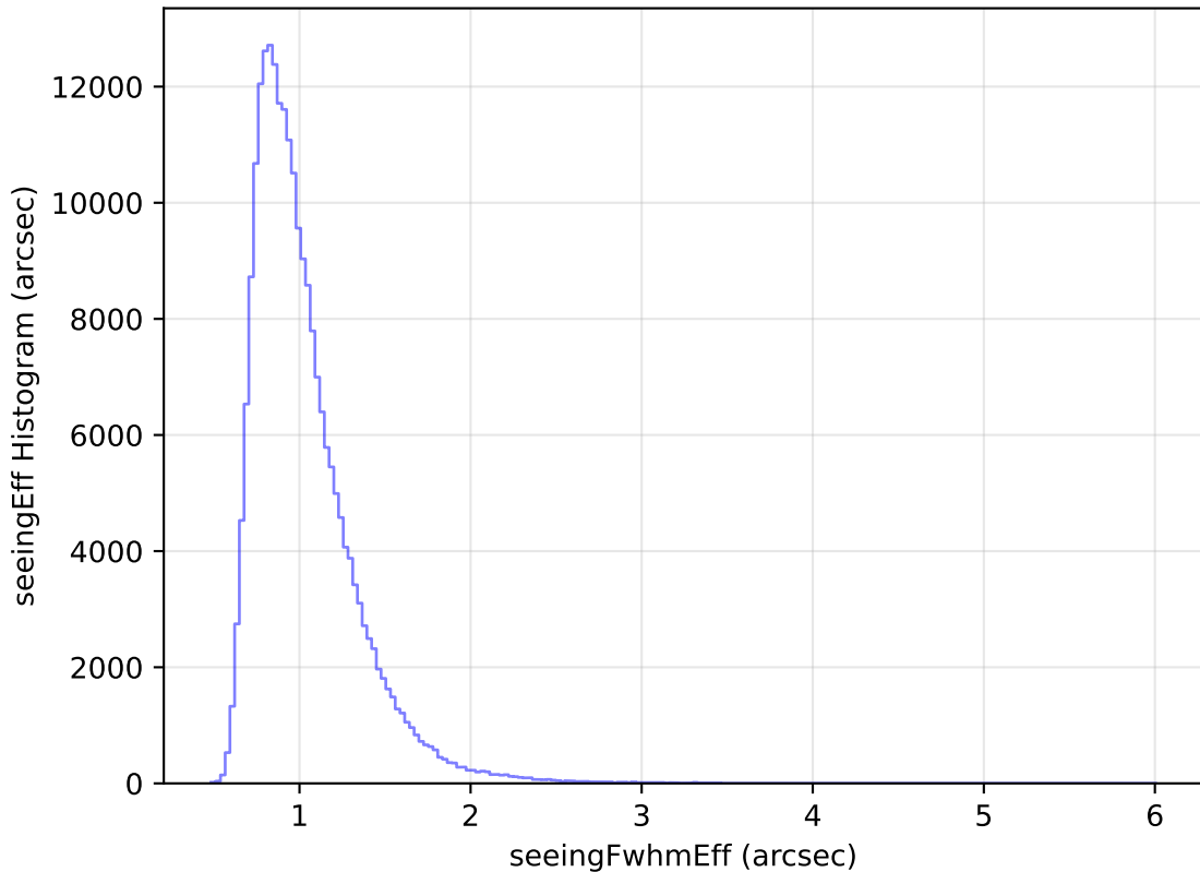
too_elab_r32_d2_ugrizy_v3.4_10yrs Yr 1 all bands: seeingEff Histogram
