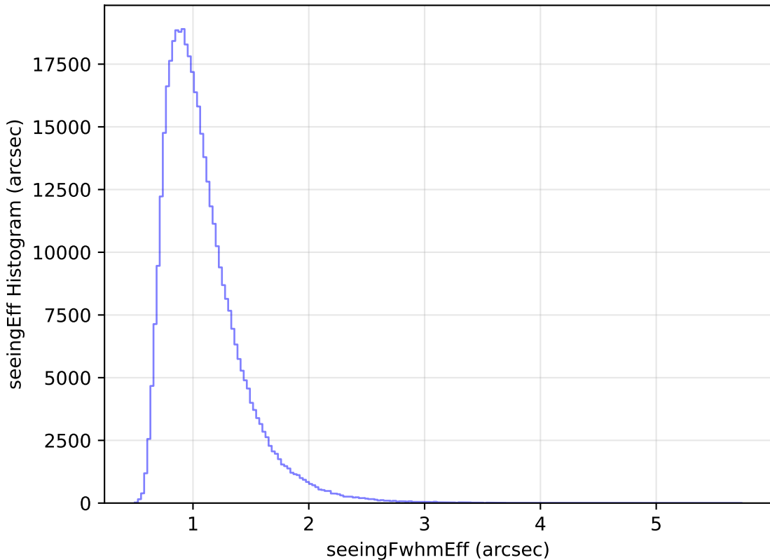
too_elab_r32_d2_ugrizy_v3.4_10yrs WFD z band: seeingEff Histogram
