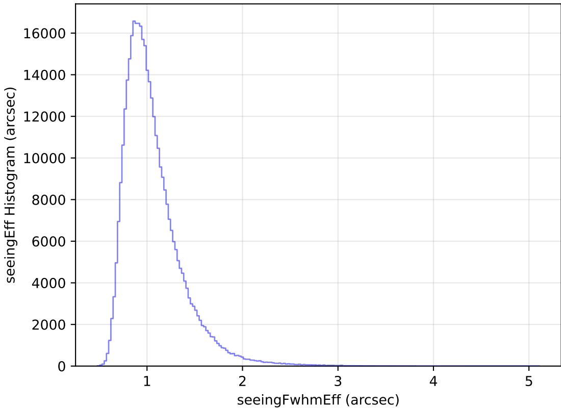
too_elab_r32_d2_ugrizy_v3.4_10yrs WFD y band: seeingEff Histogram
