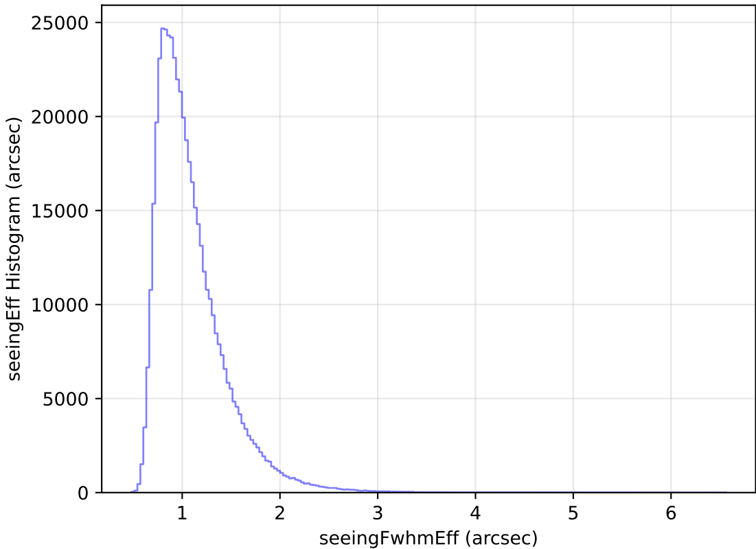
too_elab_r32_d2_ugrizy_v3.4_10yrs WFD i band: seeingEff Histogram
