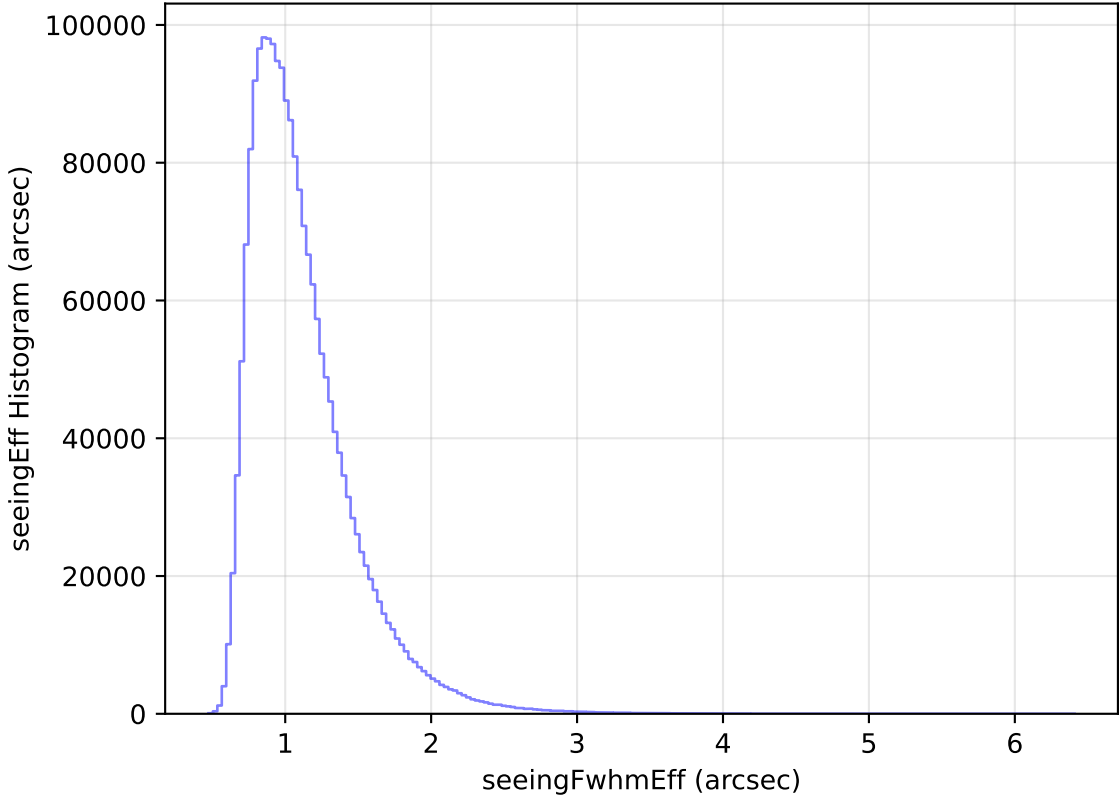
too_elab_r32_d2_ugrizy_v3.4_10yrs WFD all bands: seeingEff Histogram
